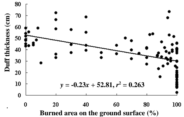
Fig. 2. Relationship between burned area and mean duff thickness in 80 1 m \times 1 m quadrats.
